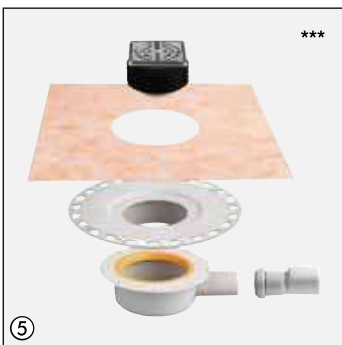
Schlüter®-KERDI-DRAIN-BASE (1 stuk) incl. rooster-/frameset
