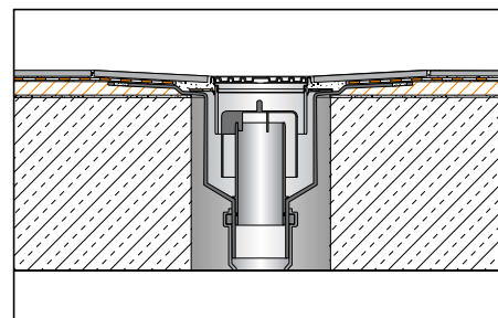
Verticale afwatering
