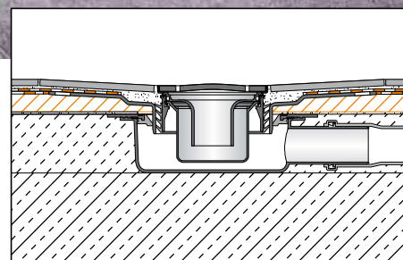
Horizontale afwatering
