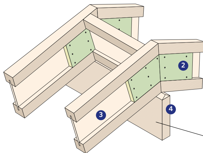
Nokbalk oplegging
