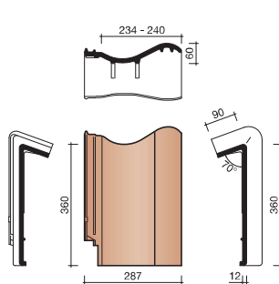
8500 CHAPERONPAN
