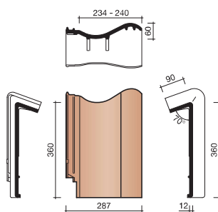
8500 CHAPERONPAN
